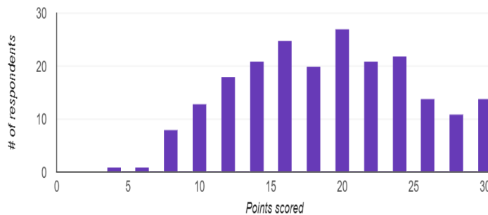
Total points distribution
