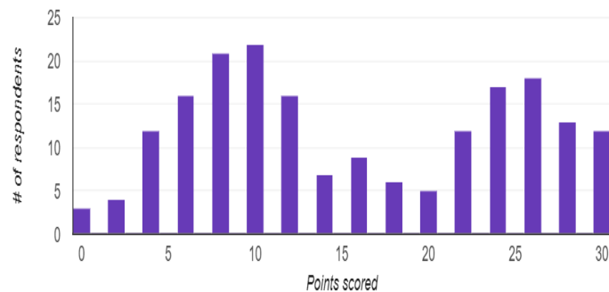
Total points distribution
